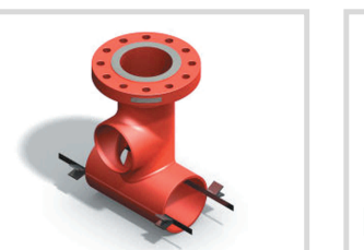
HTW Hot Tap 3-Way Split Tee
