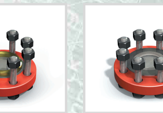
BFS Blind Flange Set - Ring Type Joint
