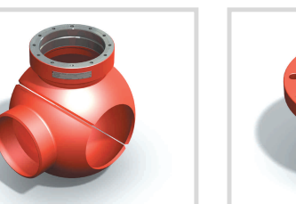
SLC Spherical Leaflock Tee
