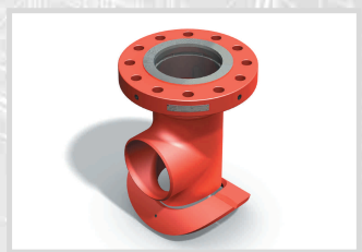
STN Seglock 3-Way Nozzle with Reinforcing Pad
