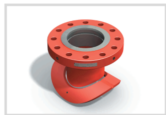
SNR Seglock Flange on Nozzle with Reinforcing Pad
