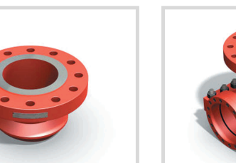
HFW Hot Tap Flange on Weldolet
